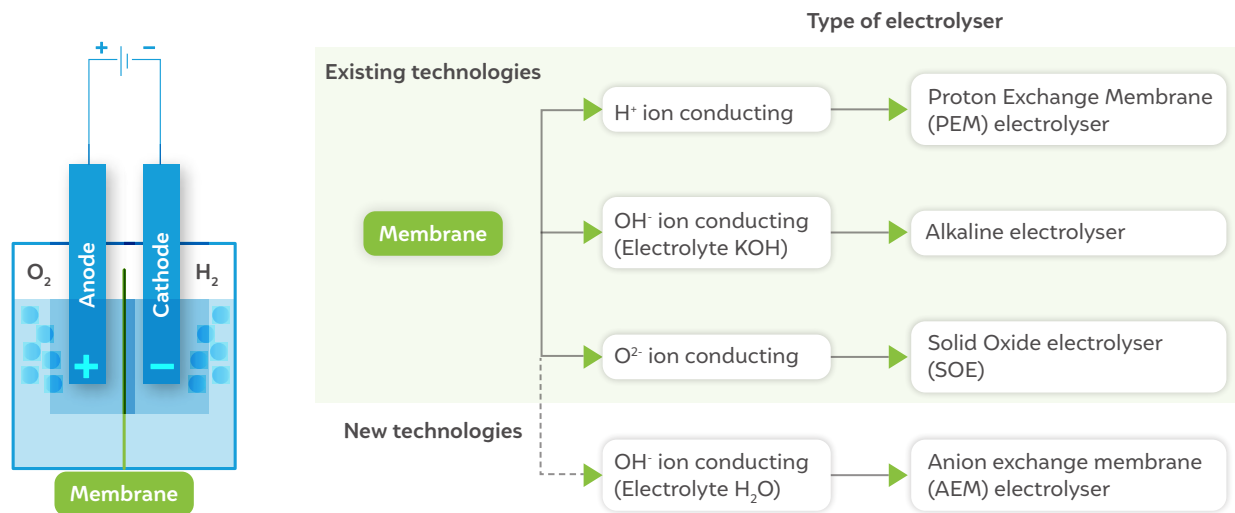
Figure 1 Electrolysers are categorised based on the selective conductivity of the membrane
