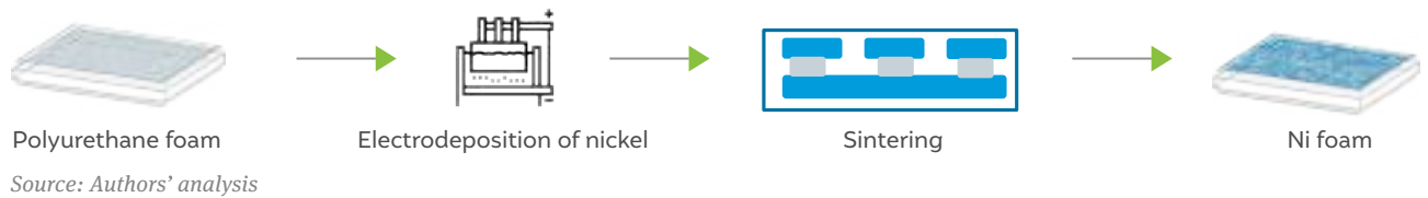
Figure 23 Anode and cathode porous transport layer manufacturing process
