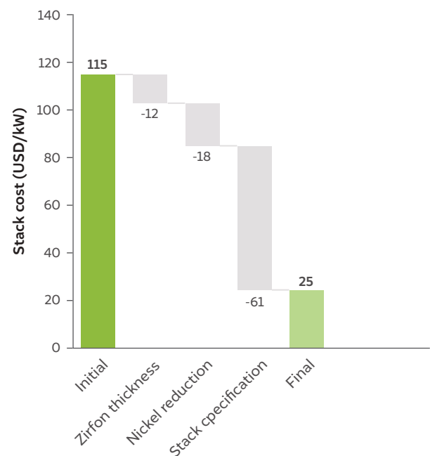
b) Stack cost reduction for alkaline electrolyzers
