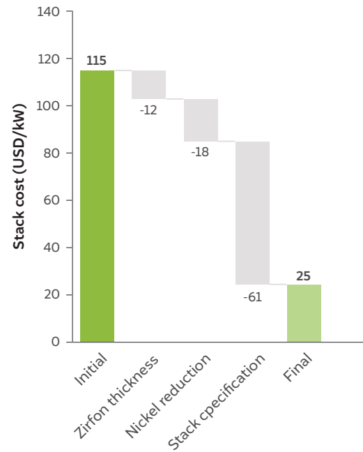
b) Stack cost reduction for alkaline electrolyzers
