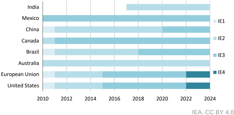
Evolution of minimum energy performance standards for industrial motors in key markets, 2010-24
