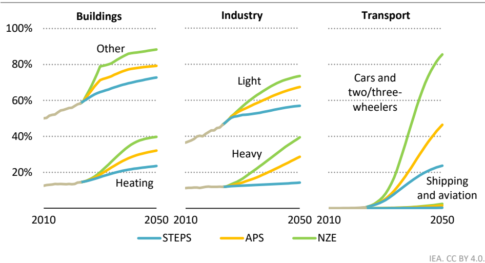
Figure 3.8 ▶ Share of electricity in total final consumption by end-use sector and scenario, 2010-2050
