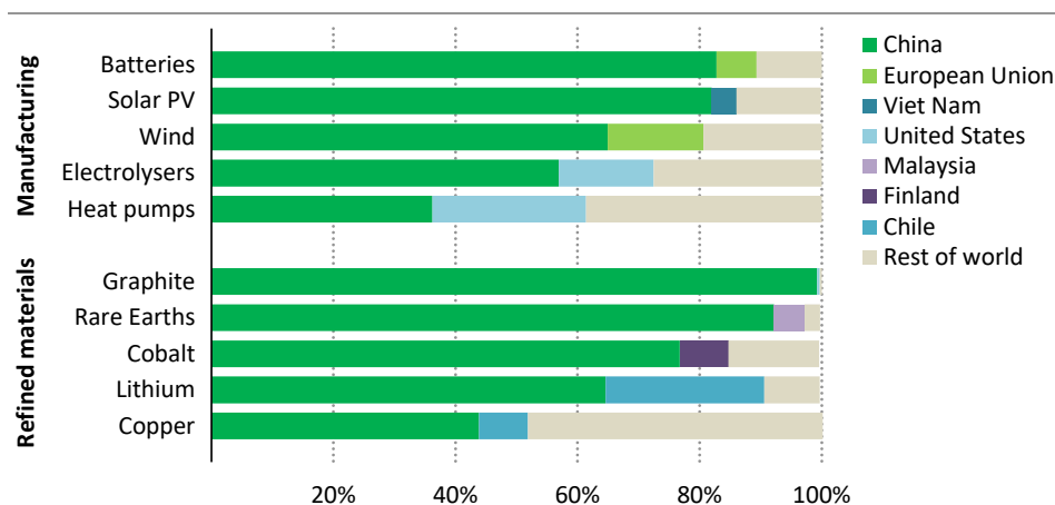
Figure 2.7 ▶ Share of clean energy technology supply chains, 2023
