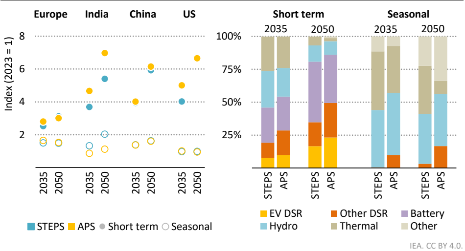
Figure 5.9 ▶ Power system flexibility needs in selected regions and global flexibility supply in the STEPS and APS
