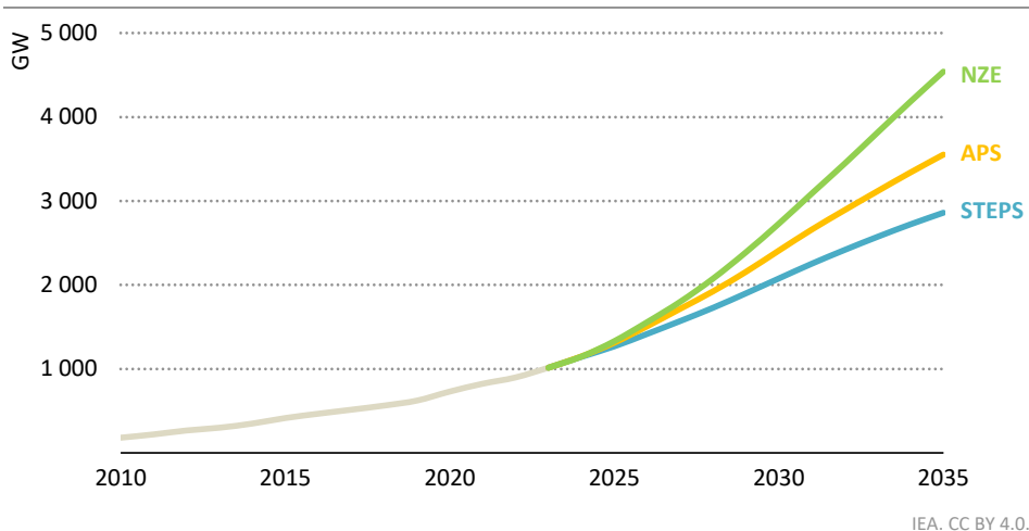
Figure 3.44 ▶ Wind power capacity by scenario, 2010-2035
