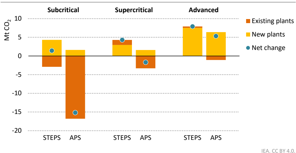
Figure 6.15 ▶ Average annual change in coal-fired power plant emissions by technology type in Southeast Asia in the STEPS and APS, 2023-35
